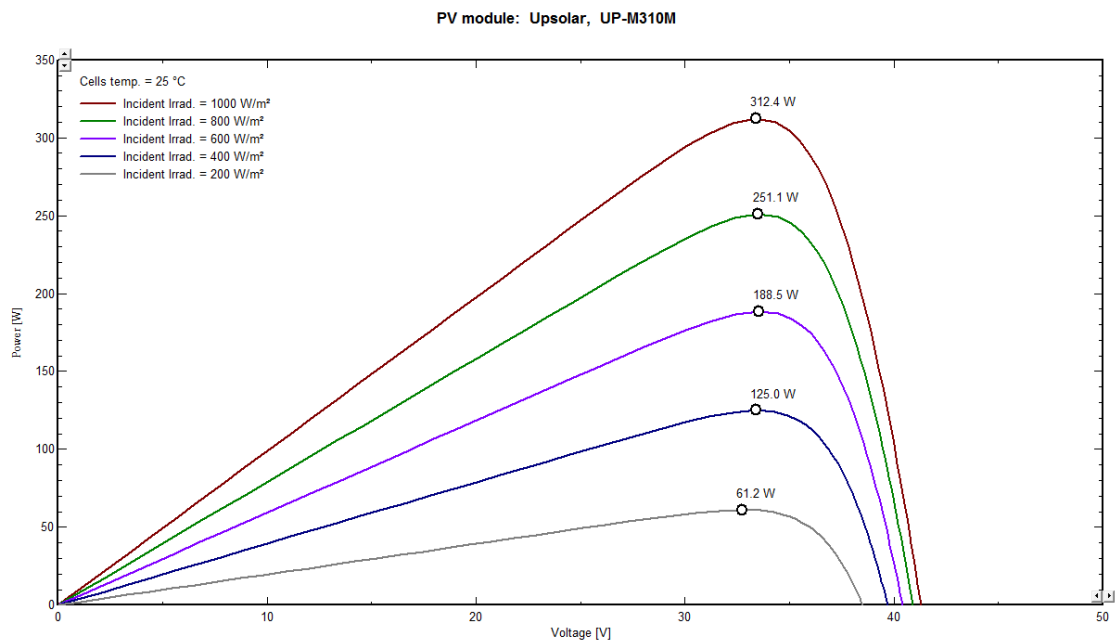
P-V curve of UP-M310M for different irradiance levels
