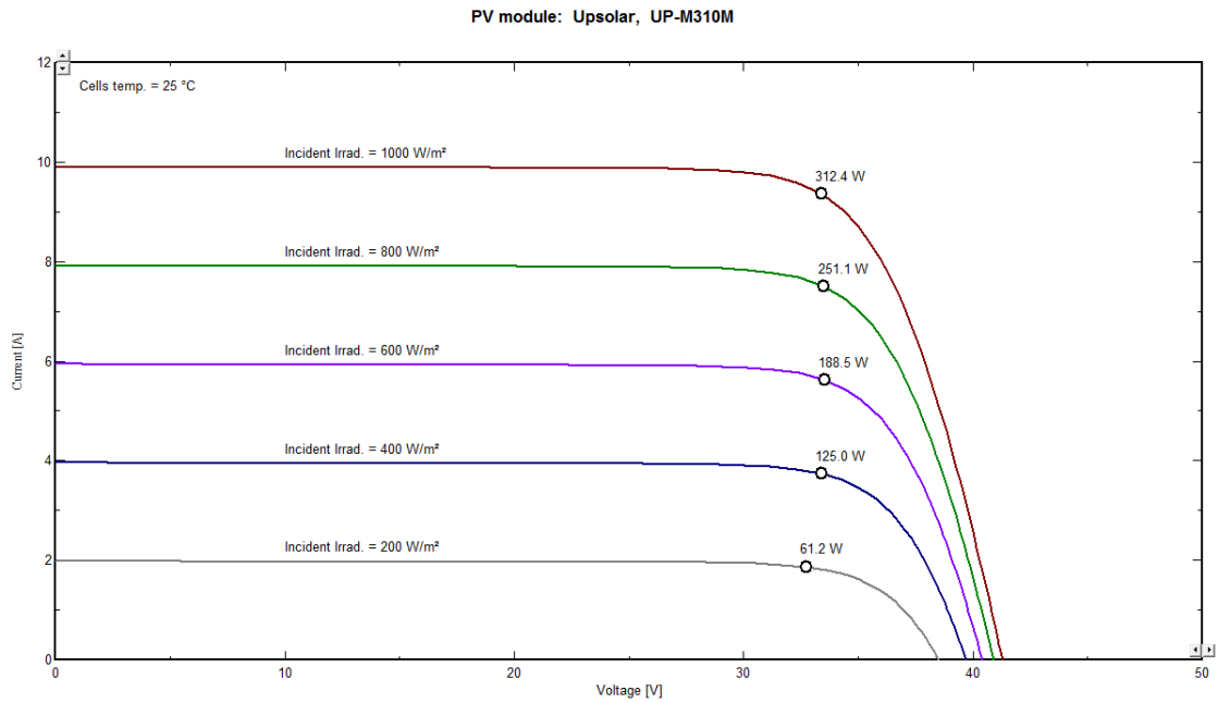
I-V curve of UP-M310M for different irradiance levels
